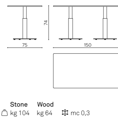
IS 75150 Table 75x150x74 cm Tavolo 75x150x74 cm Table 75x150x74 cm
