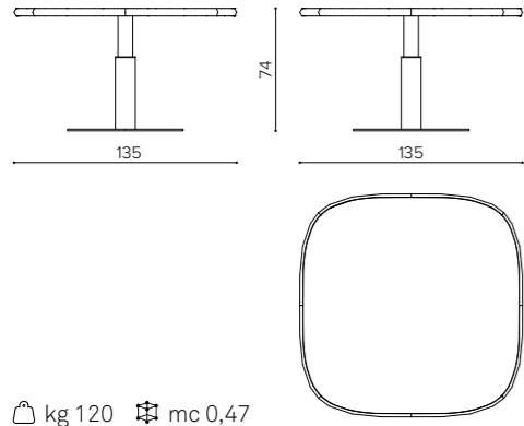
IS 135 Table 135x135x74 cm Tavolo 135x135x74 cm Table 135x135x74 cm
