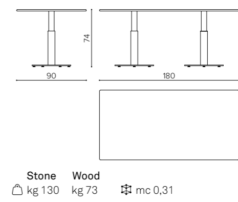
IS 90180 Table 90x180x74 cm Tavolo 90x180x74 cm Table 90x180x74 cm
