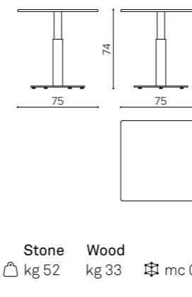
IS 7575 Table 75x75x74 cm Tavolo 75x75x74 cm Table 75x75x74 cm
