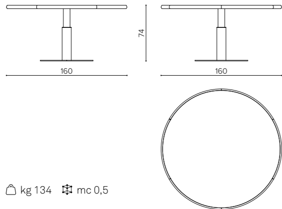
IS 160 Table Ø160x74 cm Tavolo Ø160x74 cm Table Ø160x74 cm
