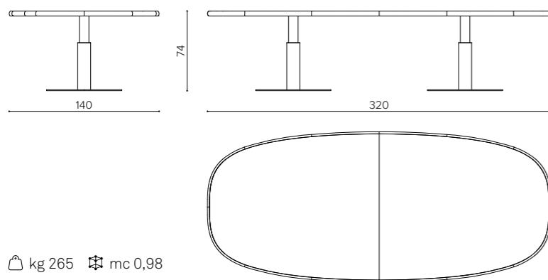
IS 320 Table 140x320x74 cm Tavolo 140x320x74 cm Table 140x320x74 cm
