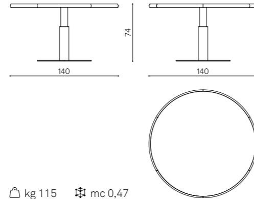
IS 140 Table Ø140x74 cm Tavolo Ø140x74 cm Table Ø140x74 cm
