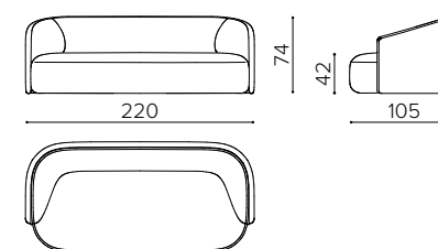
SY 2000 2-seater sofa divano 2 posti canapé 2 places
