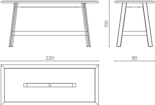
ZU22090H table 220x90x100cm tavolo 220x90x100cm table 220x90x100cm
